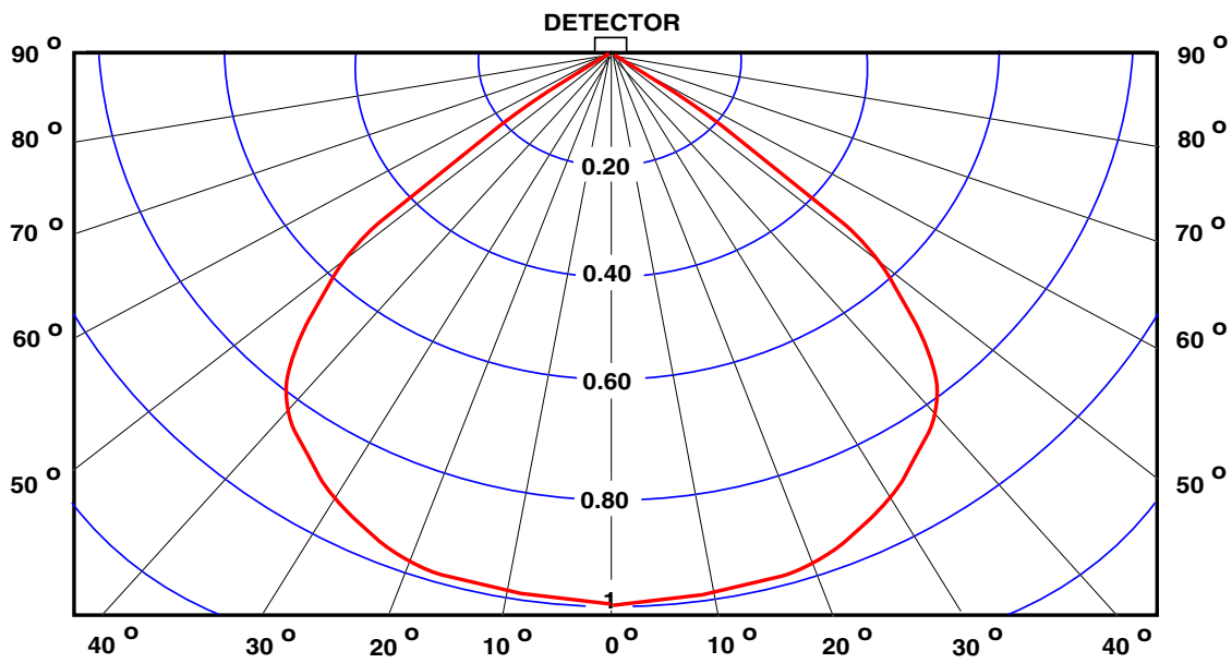
Fig. 6: Relative Range vs Angle of Incidence
